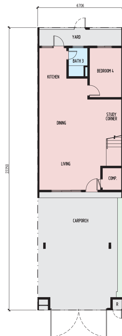
Ground floor
